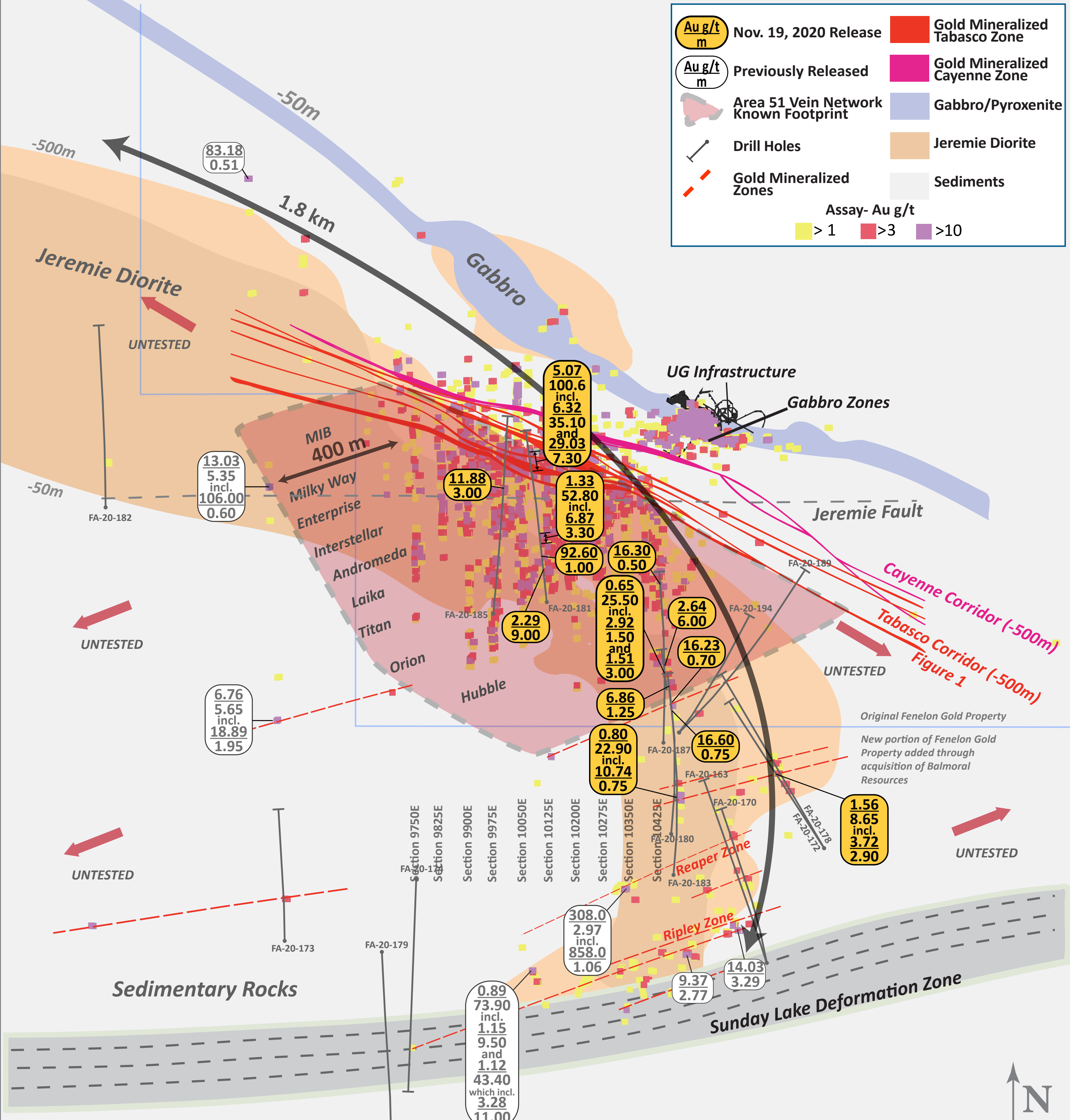
Fenelon Gold System Plan View November 19, 2020
