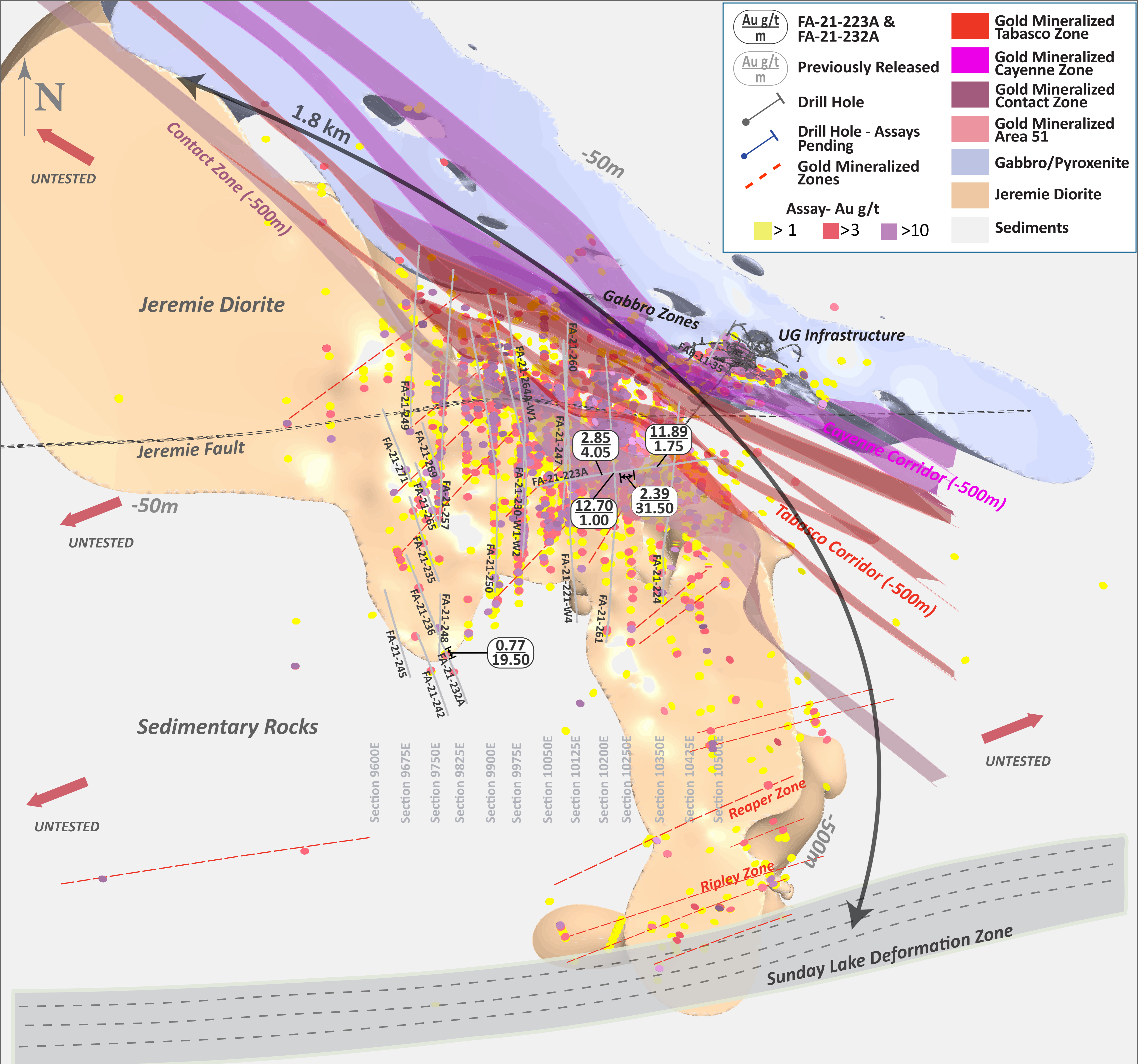
Fenelon Gold System Plan View June 29, 2021
